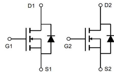
Schematic Diagram
